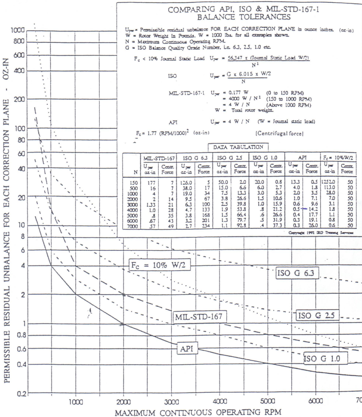
Figure 7 Comparison of API, ISO & MIL-STD-167-1 Balance Tolerances.
